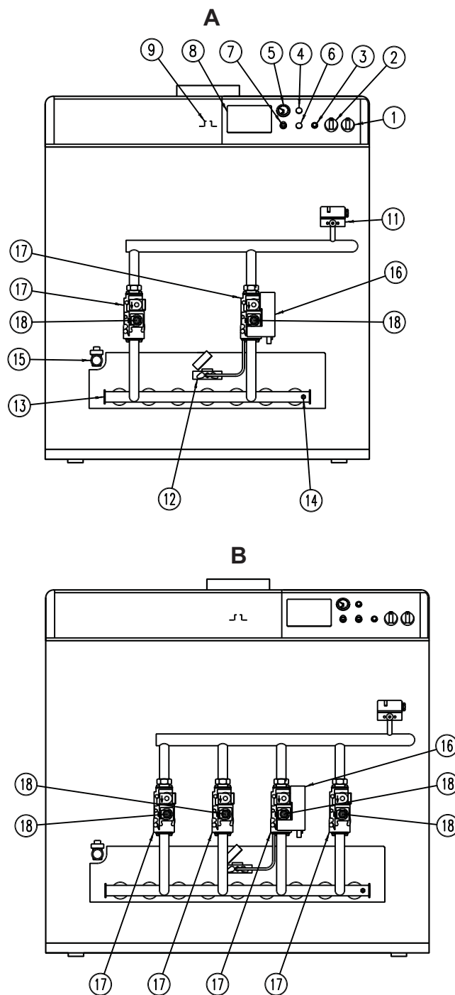
fig. 11 - General view and main components
